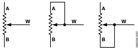
Figure 36. Rheostat Mode Configuration
